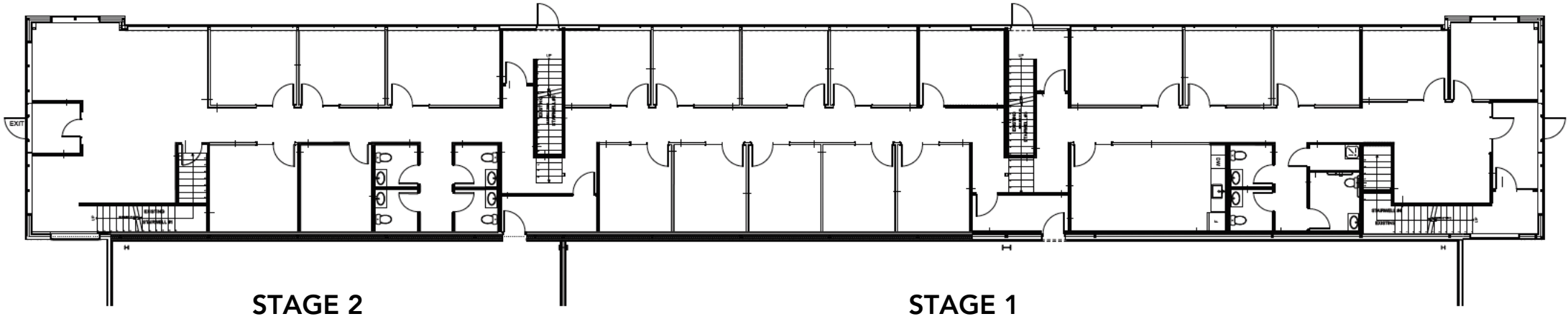
MAIN FLOOR 6,500 sq.ft.
